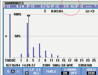
Figure 6 - Hz inter-harmonics
