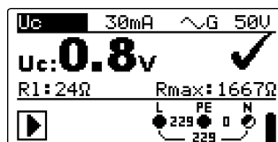
Figure 5.18: Example of contact voltage measurement results
