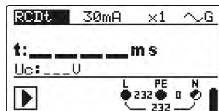
Figure 5.16: Test RCD
