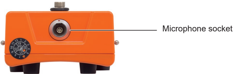
Fig. 5: RT 200 transmitter, back
