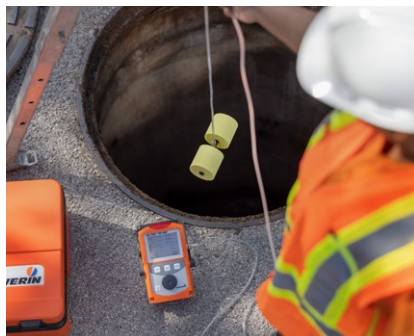
Measuring shafts
