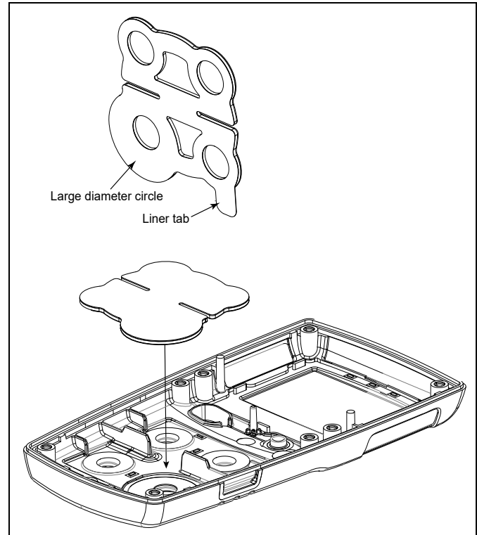
Figure 10. Liner Tab
