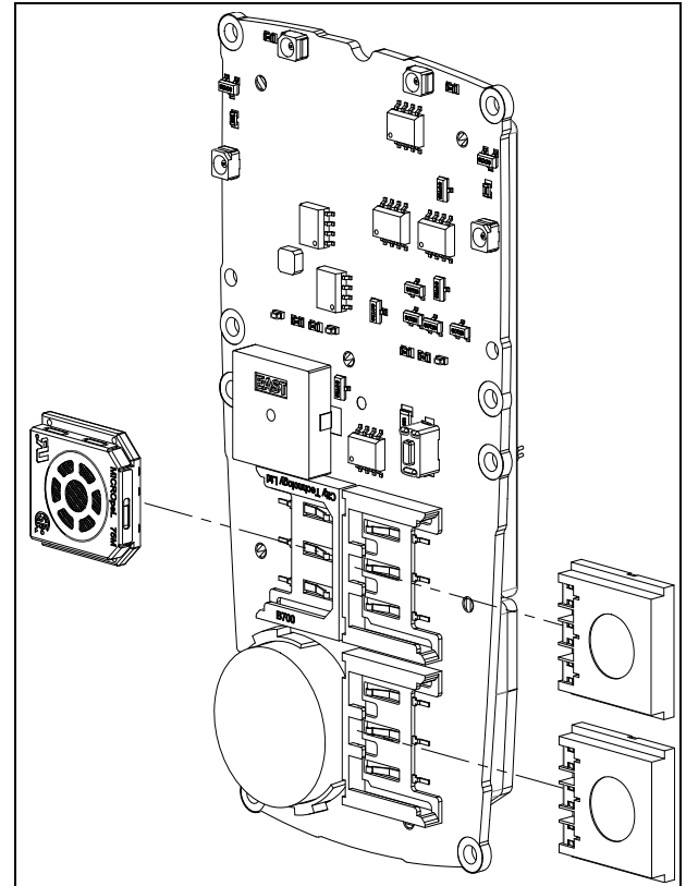
Figure 11. Sensor Positioning
