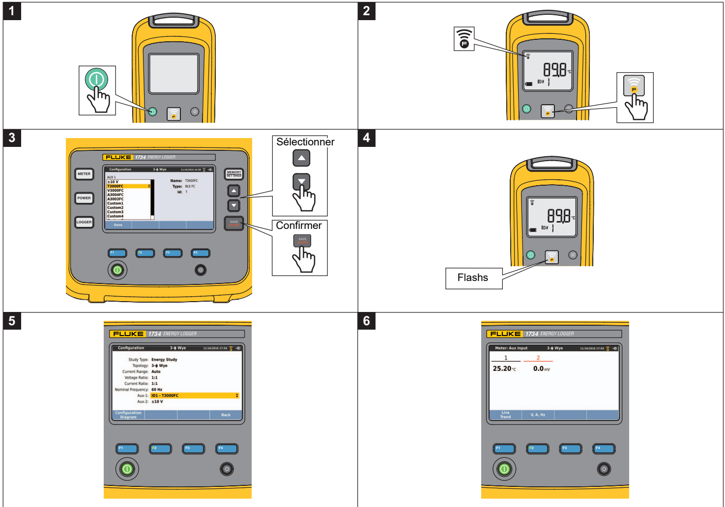
Figure 10. Connexion sans fil aux modules Fluke Connect
