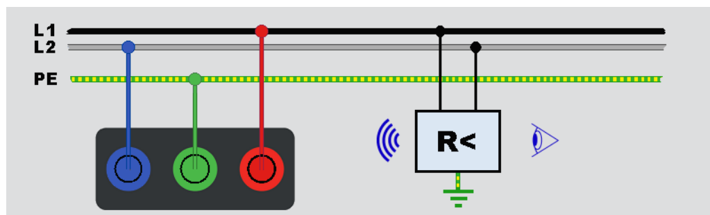
Figure 22. Test IMD n°1
